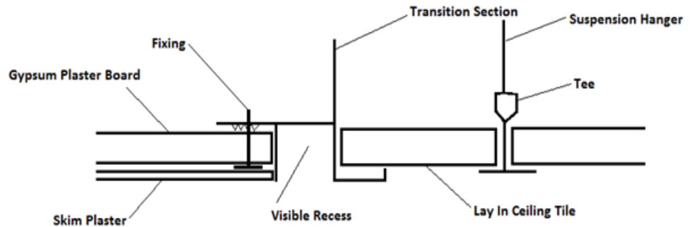
CPW TRANSITION SECTION APPLICATION DIAGRAM
